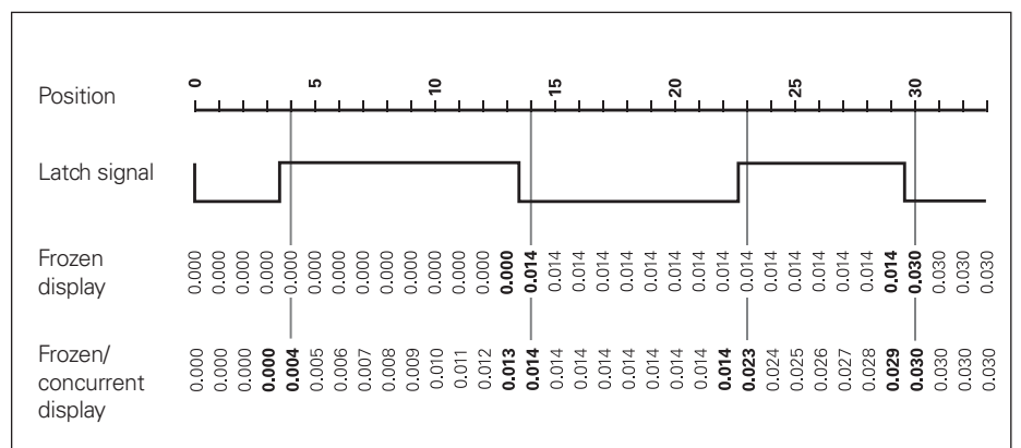
Function of the display freeze features
